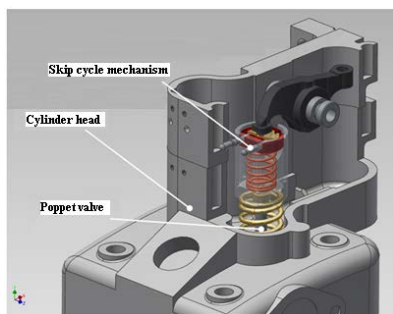
Figure 5. Cylinder head and location of skip cycle mechanism
